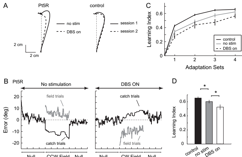
Figure 3. Effect of DBS on motor adaptation. (A) Average catch trial trajectories of a DBS patient and a control subject. Trials were taken from the last adaptation set of each session and were rotated to a canonical direction before averaging. Trials from the session where a clockwise force field was given are inverted for ease of visual comparison. (B) Performance of a DBS patient with stimulation (left) and with out stimulation (right). Shown here are moving averages (window size = 15) of angular error for all trials in each session. The patient achieved significantly higher catch trial errors and lower field trial errors with DBS off than DBS on. (C) Average learning index for each adaptation set is shown for the control group and each stimulation condition for the patient group. Error bars are standard errors. (D) Summary of performance: the average learning index over the last 2 adaptation sets for each subject group. With no stimulation, patients showed reduced learning index compared with control subjects ( P = 0.025 ). With DBS turned on, an additional reduction in learning was observed ( P = 0.024 ).
